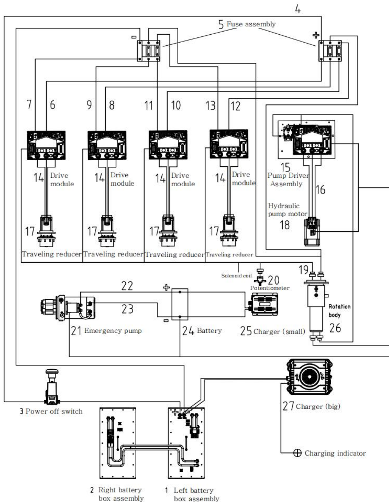
Figure6-1 Cable Assembly
