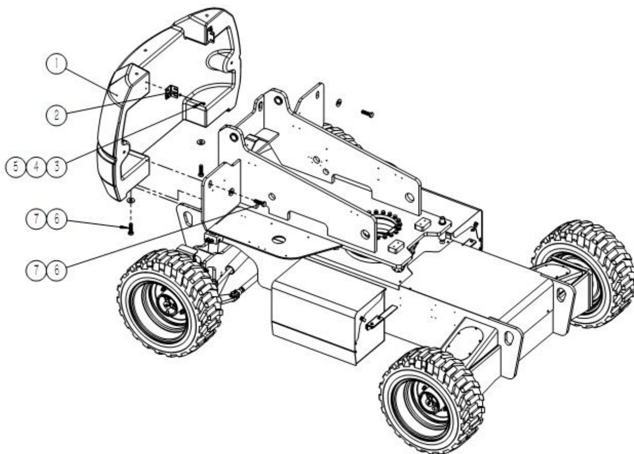
Figure2-2 Counterweight and rotating frame assembly
