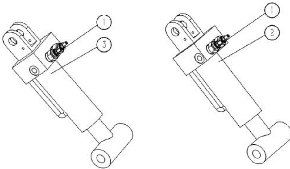
Figure5-3 Oscillation cylinder assembly
