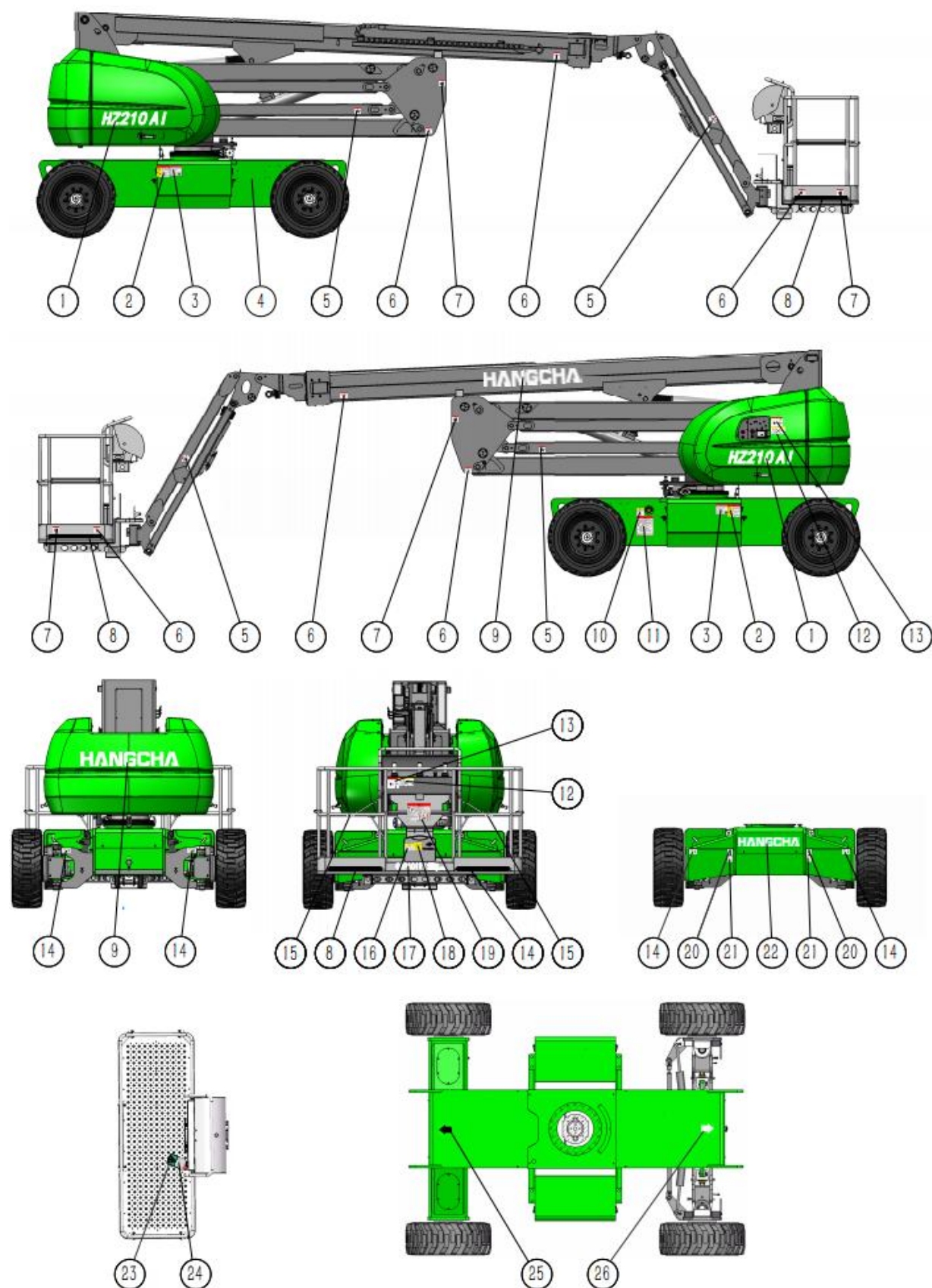
Figure7-1 adhesive signs
