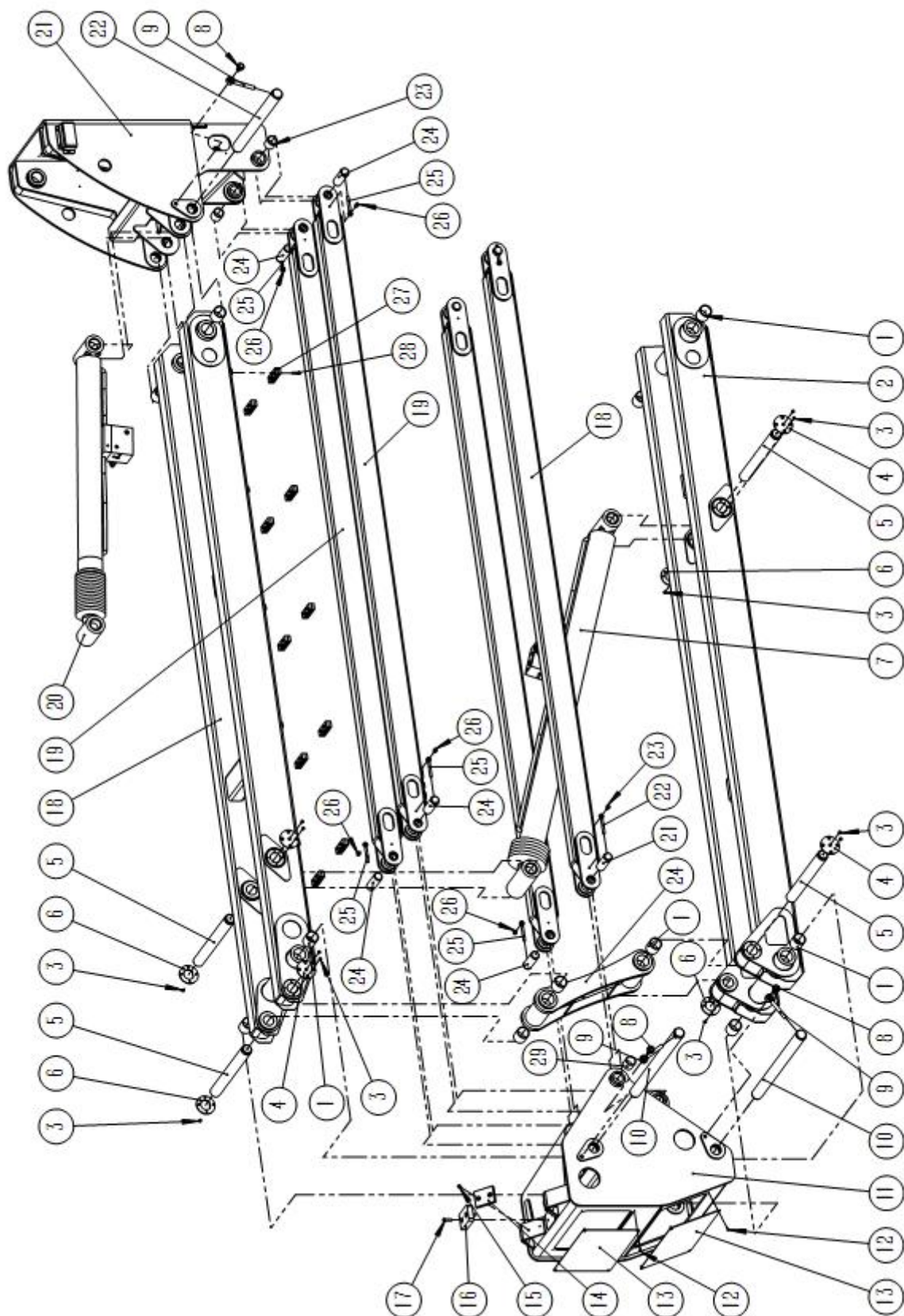
Figure3-2 Boom assembly
